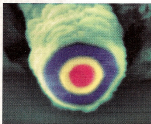
LAYERED LOOK A coaxial nanowire has a single-crystal p-type core (pink) surrounded by nanocrystalline intrinsic (yellow) and n-type (blue) layers and is topped with SiO_2 (green), as shown in this artificial-color scanning electron micrograph.
