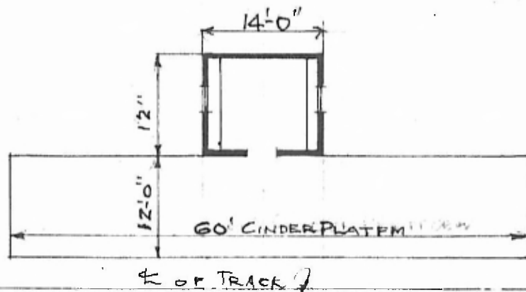
FLOOR PLAN OF SHELTER SCALE \frac{1}{16}'' = 1'-0''
