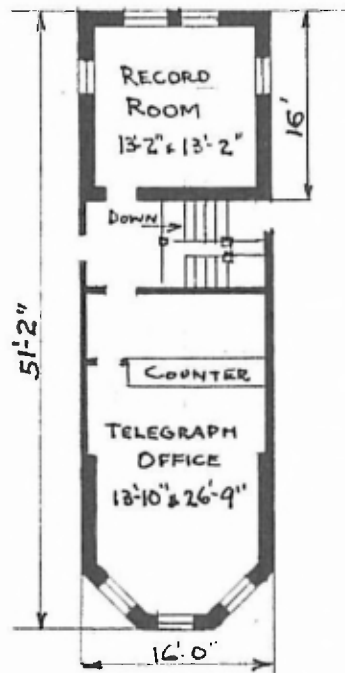
SECOND FLOOR SCALE: \frac{1}{16}'' = 1'-0''
