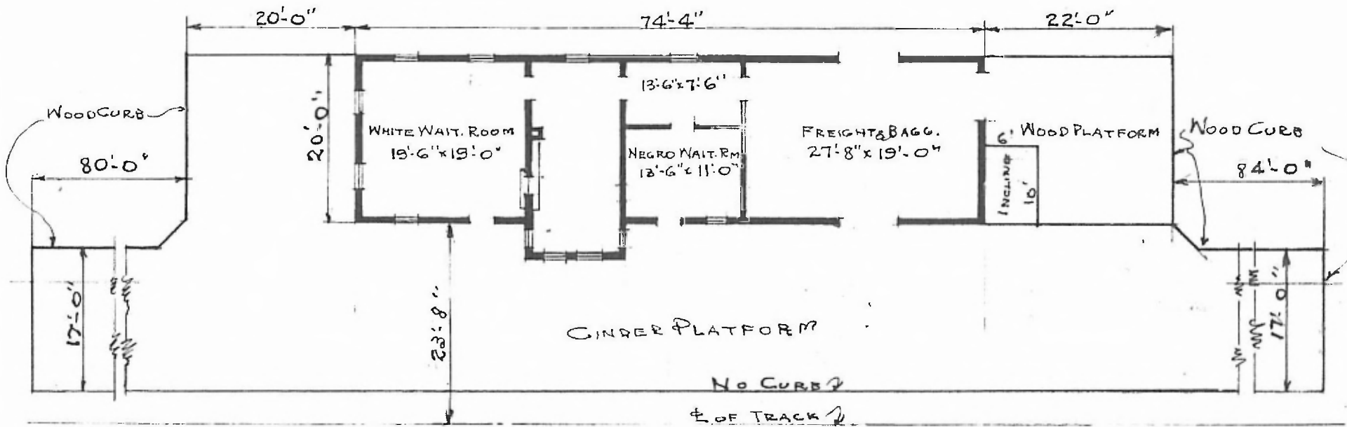
FLOOR PLAN SCALE: \frac{1}{16} " = 1'-0"
