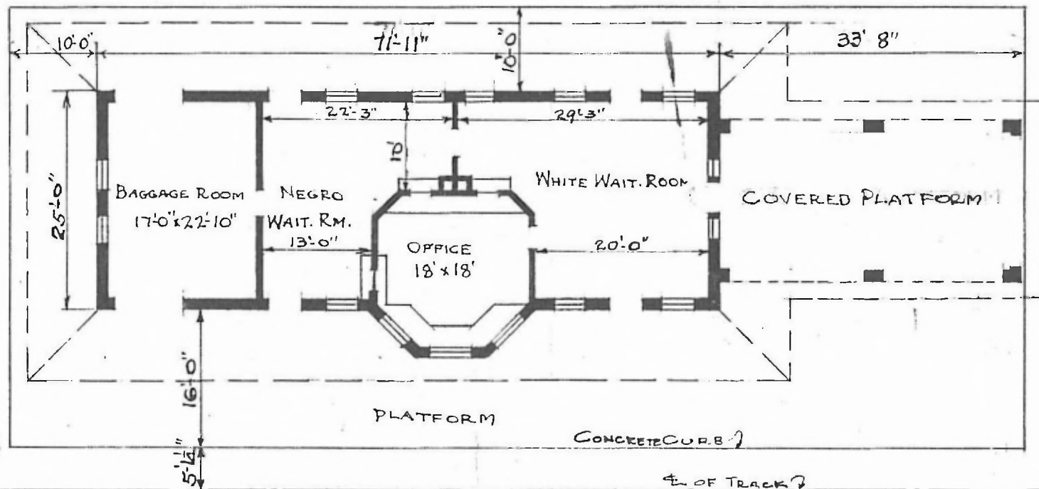
FLOOR PLAN SCALE: \frac{1}{16} " = 1'-0"
