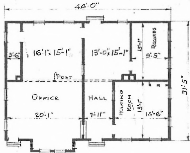
FLOOR PLAN SCALE: 1/16" = 1'-0"
