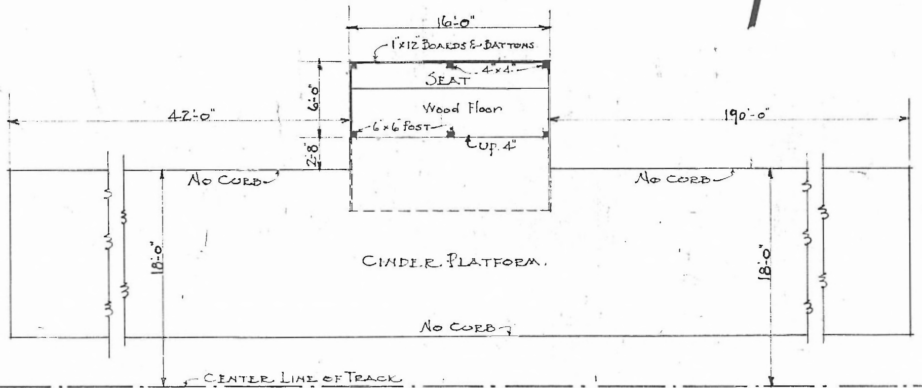
FLOOR PLAN. SCALE \frac{1}{8} " = 1'-0"
