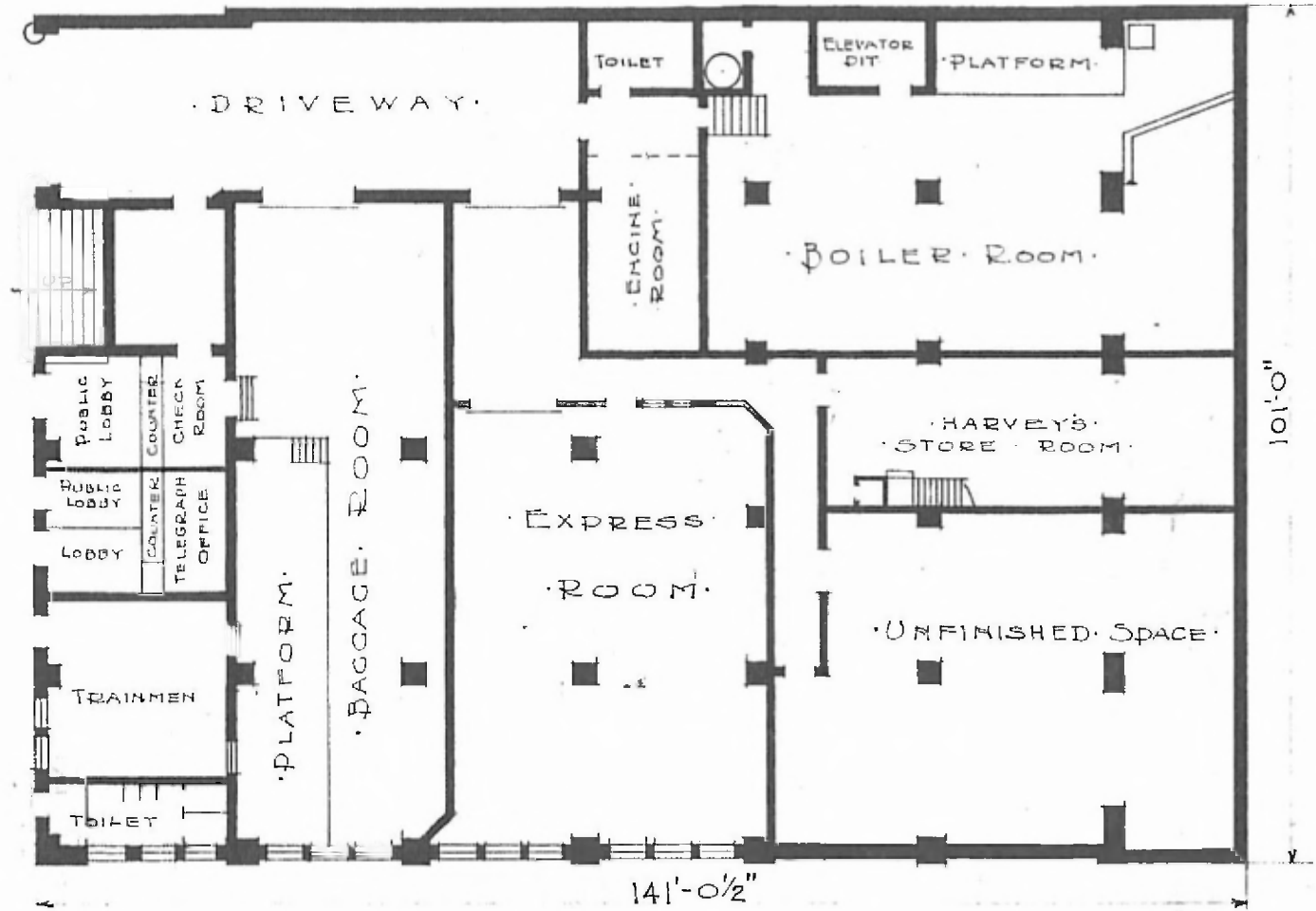
BASEMENT PLAN. SCALE \frac{3}{64} = 1'-0"
