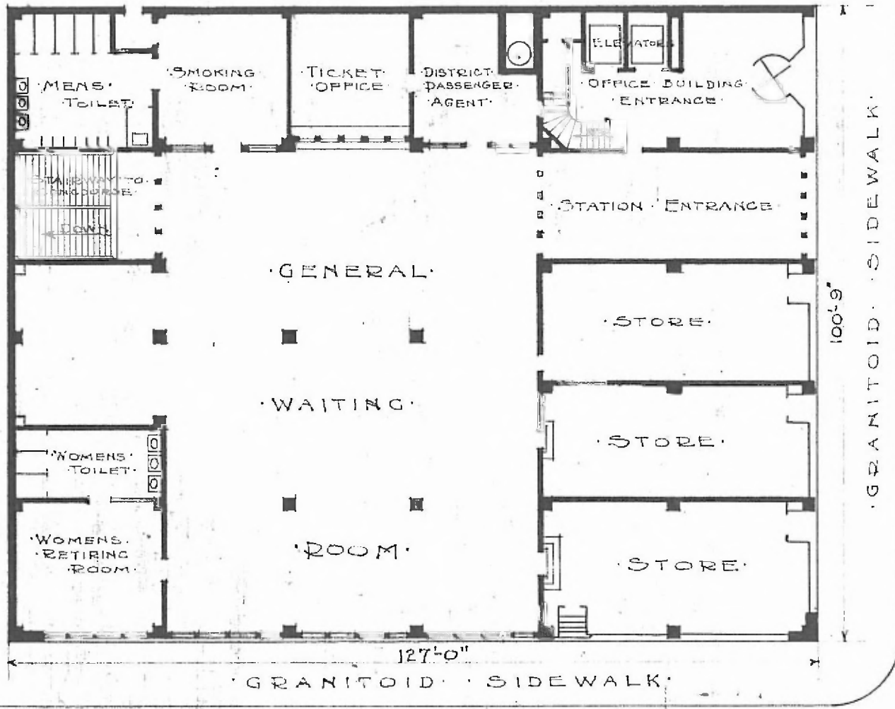
FIRST FLOOR PLAN. SCALE \frac{3}{8}'' = 1'-0''
