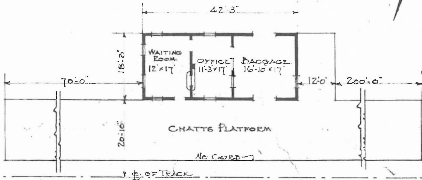
FLOOR PLAN SCALE \frac{1}{16} " = 1'-0"
