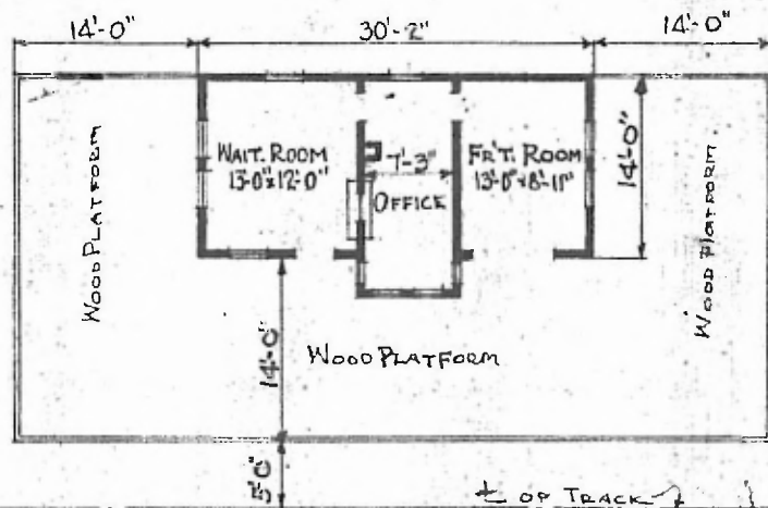
FLOOR PLAN SCALE: 1/16" = 1'-0"
