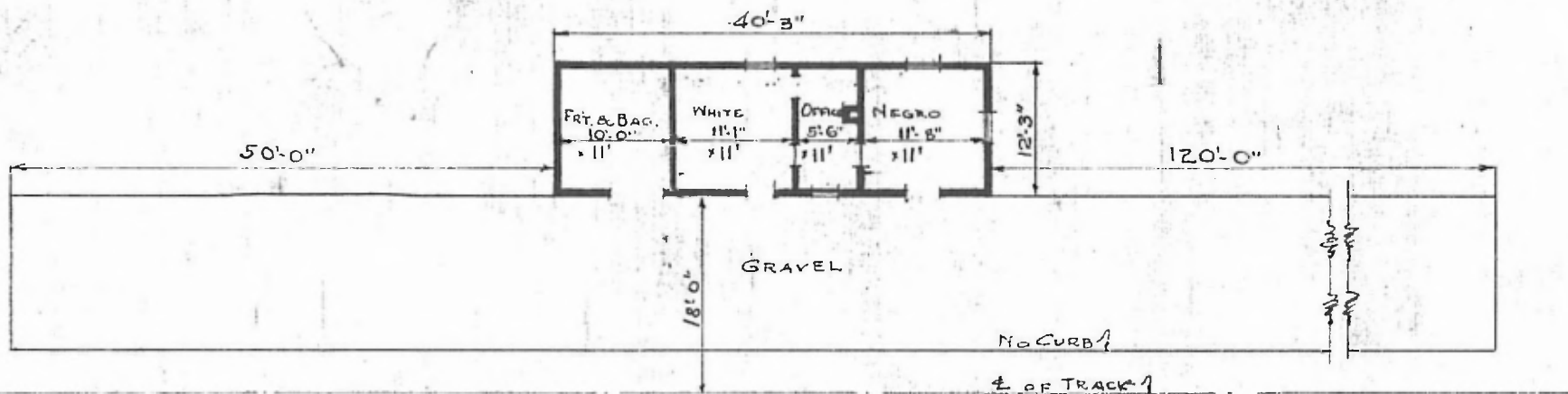
FLOOR PLAN SCALE: \frac{1}{16} " = 1'-0"
