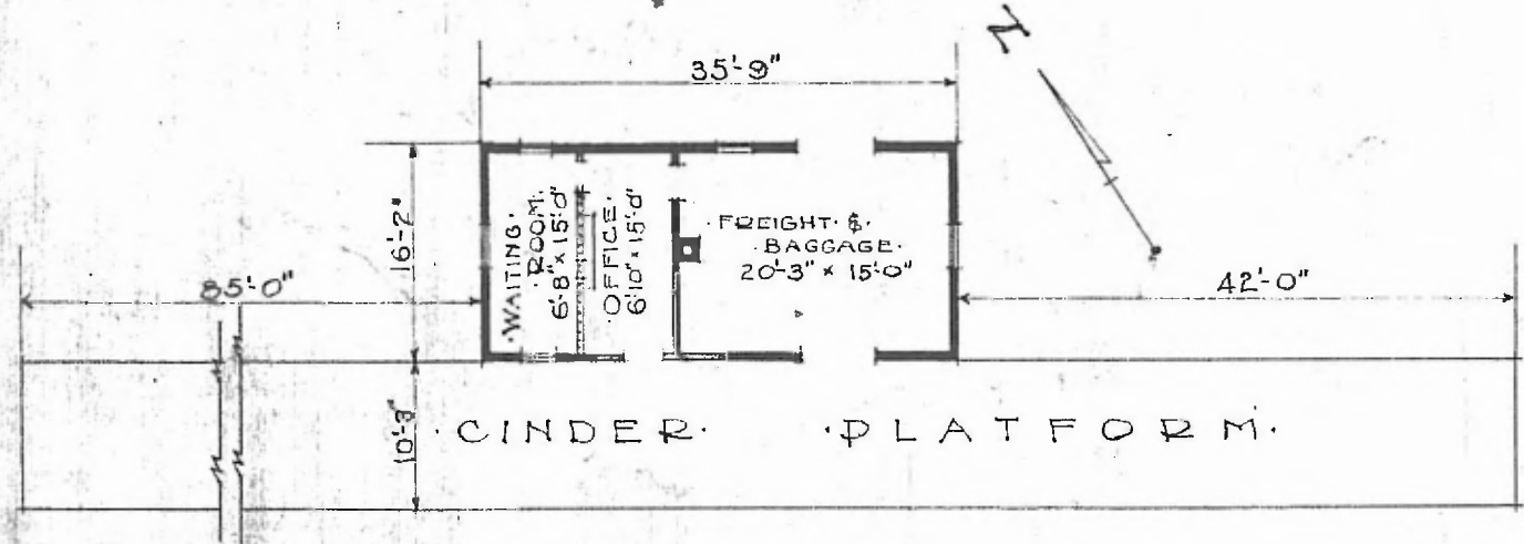
FLOOR PLAN SCALE 1/16" = 1'-0"
