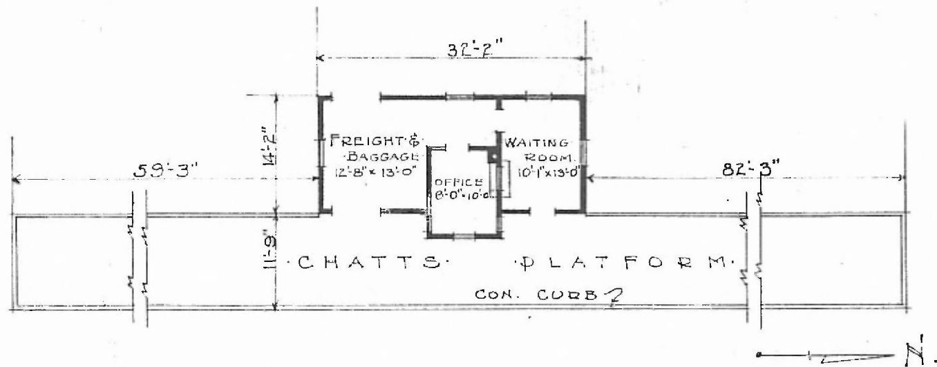
·FLOOR PLAN· SCALE \frac{1}{16} " = 1'-0"
