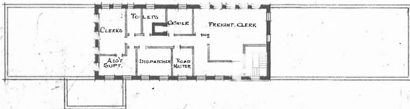
SECOND FLOOR PLAN. SCALE 24' = 1"
