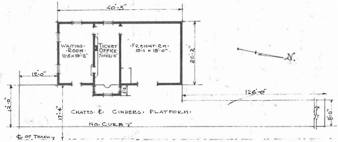
FLOOR PLAN. SCALE 1/16" = 1'-0".
