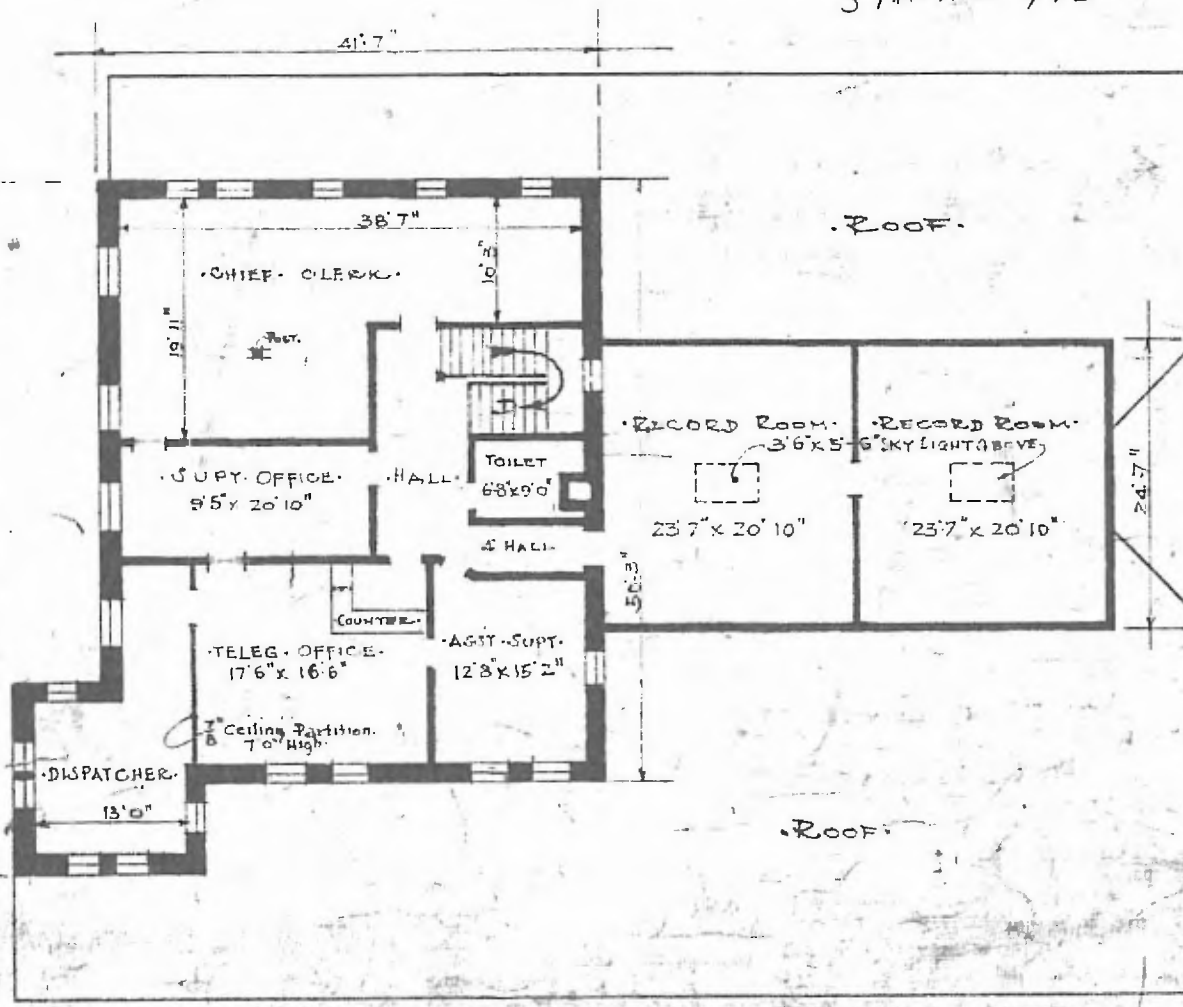
• SECOND FLOOR PLAN • SCALE 1/16" = 1'0"
