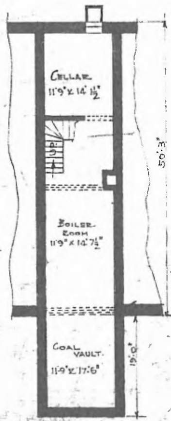
• BOILER ROOM • SCALE 1/16" = 1'0"
