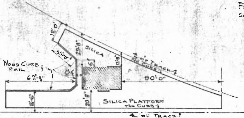
PLOT PLAN SCALE: 1" = 50'
