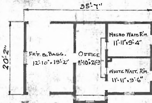
FLOOR PLAN SCALE: \frac{1}{8} " = 1'-0"
