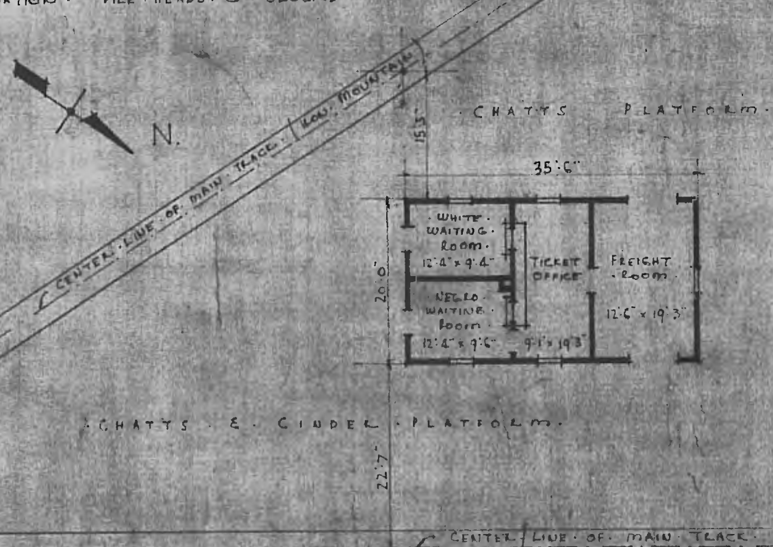
FLOOR PLAN SCALE 1/16" = 1'0"
