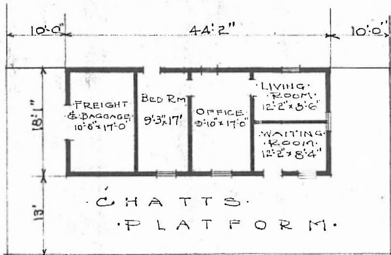
FLOOR PLAN. SCALE 1/16" = 1'-0"
