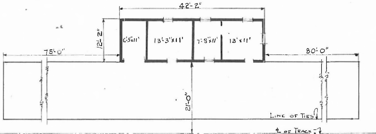
FLOOR PLAN
