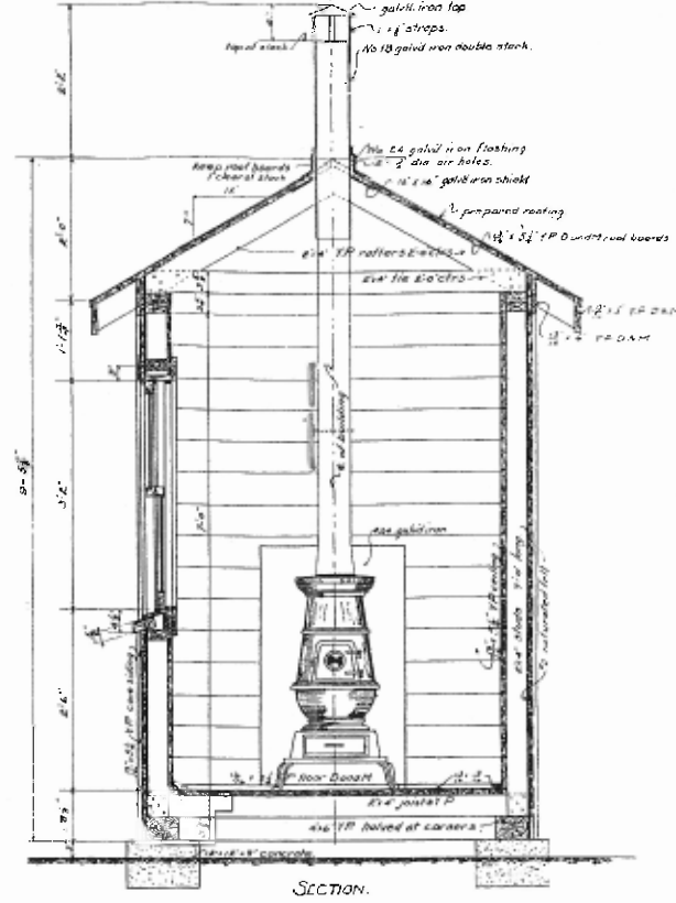
SECTION.
