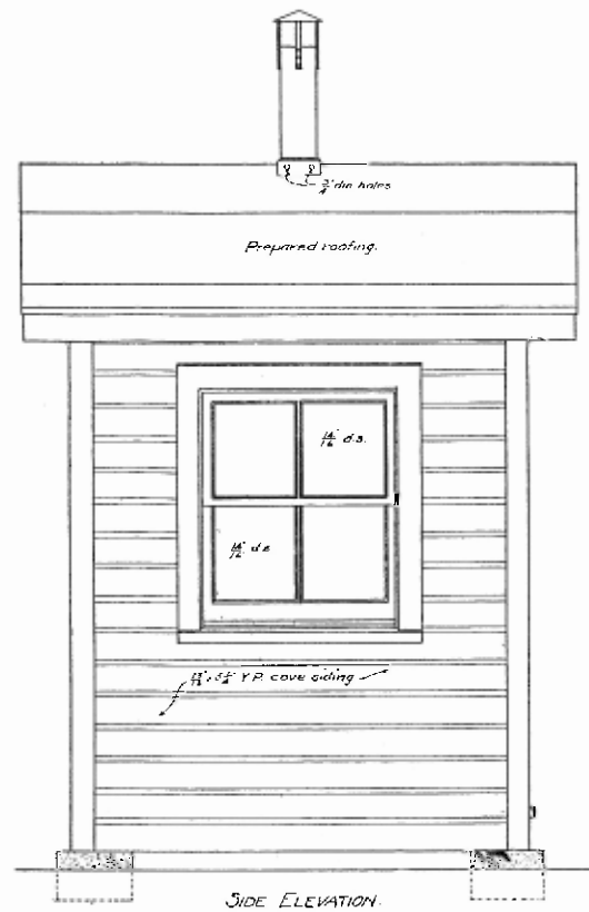
SIDE ELEVATION.
